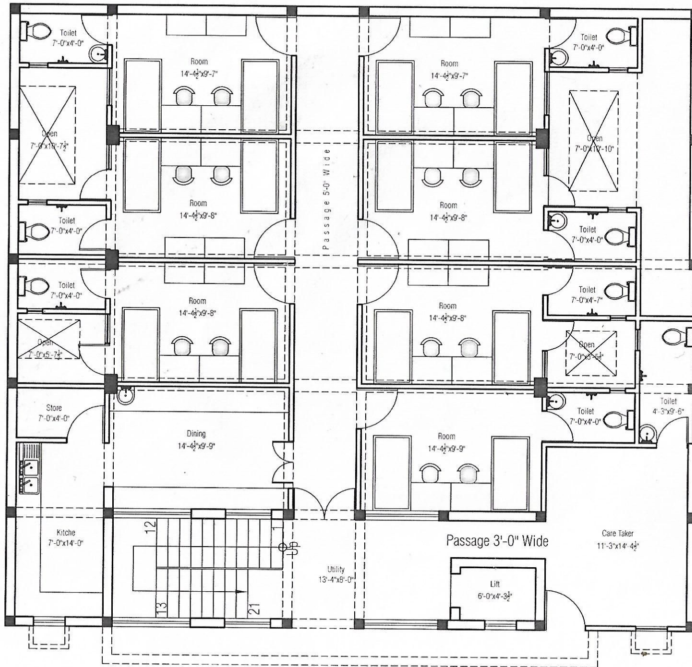
First Floor /Typical Floor For Hostel
