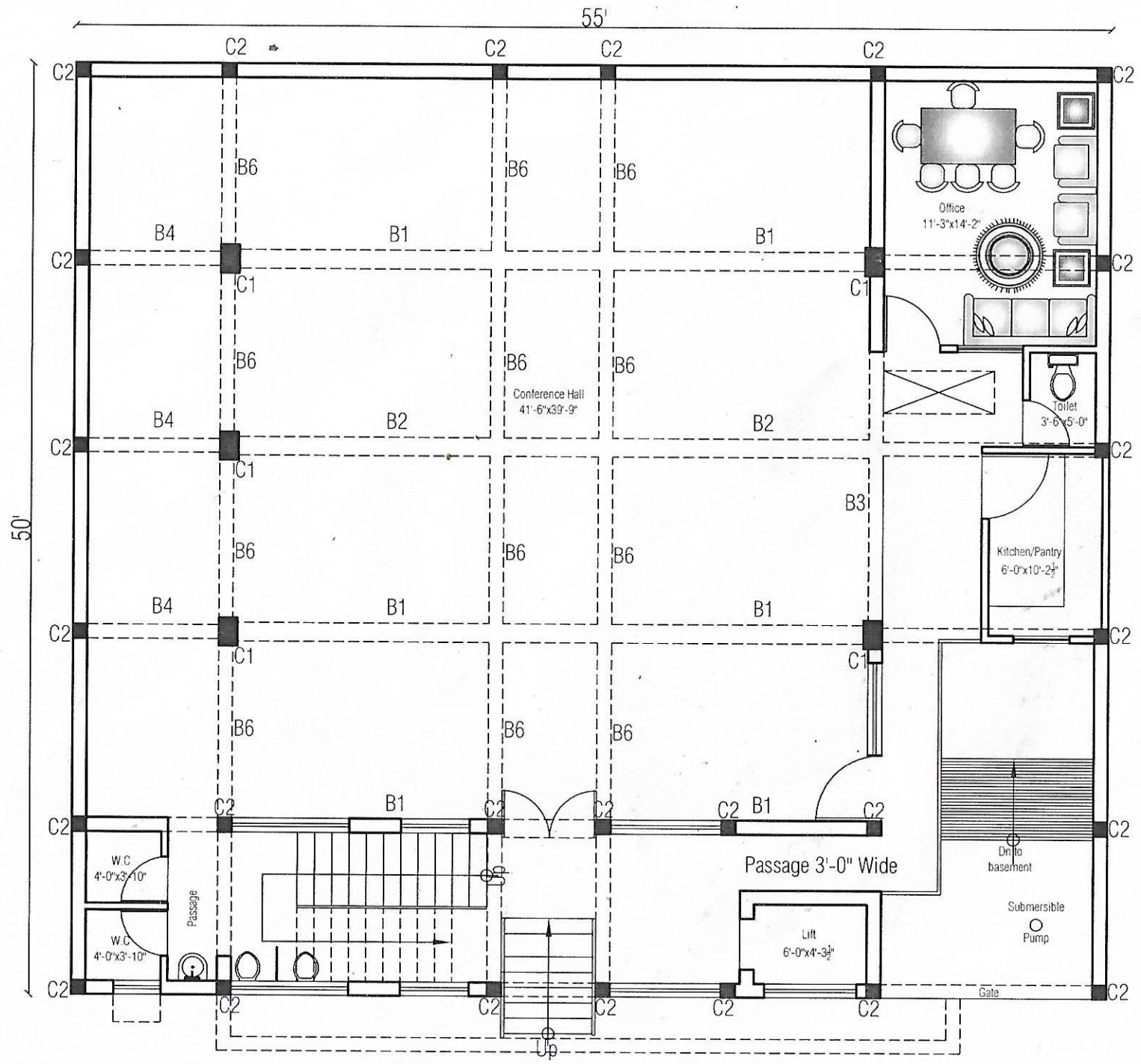
Basement /Upper Ground Floor Plan
